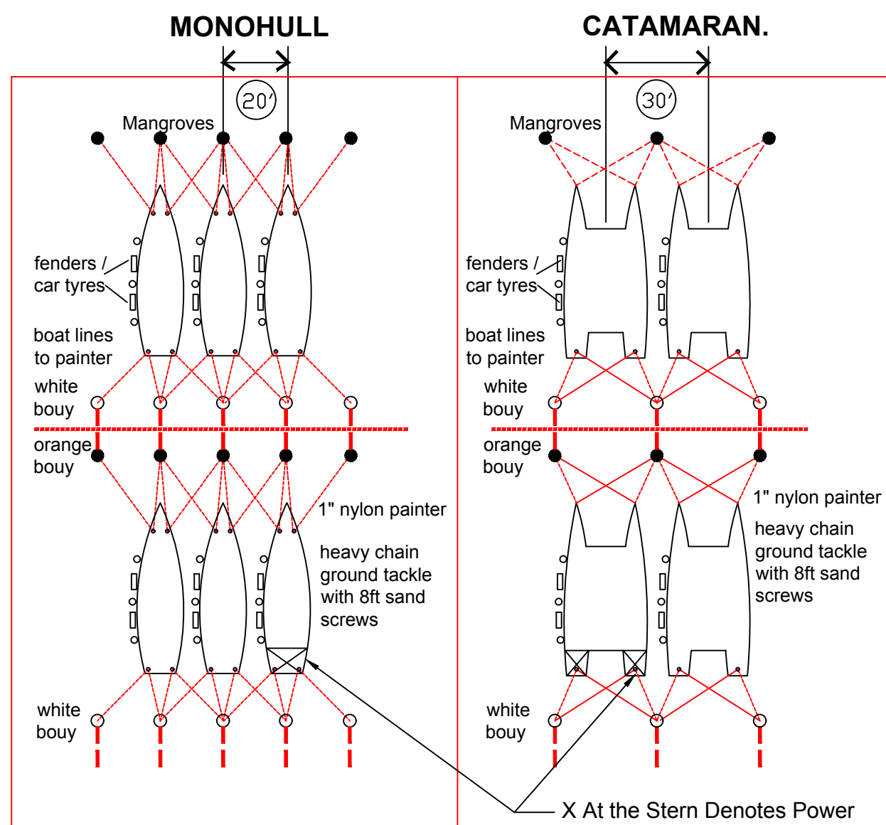
Typical mooring arrangement
